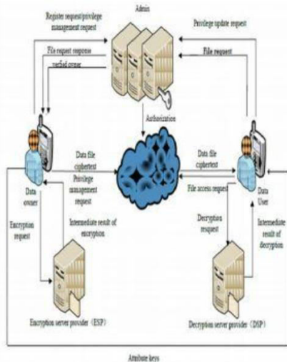
Figure 2: System Architecture
